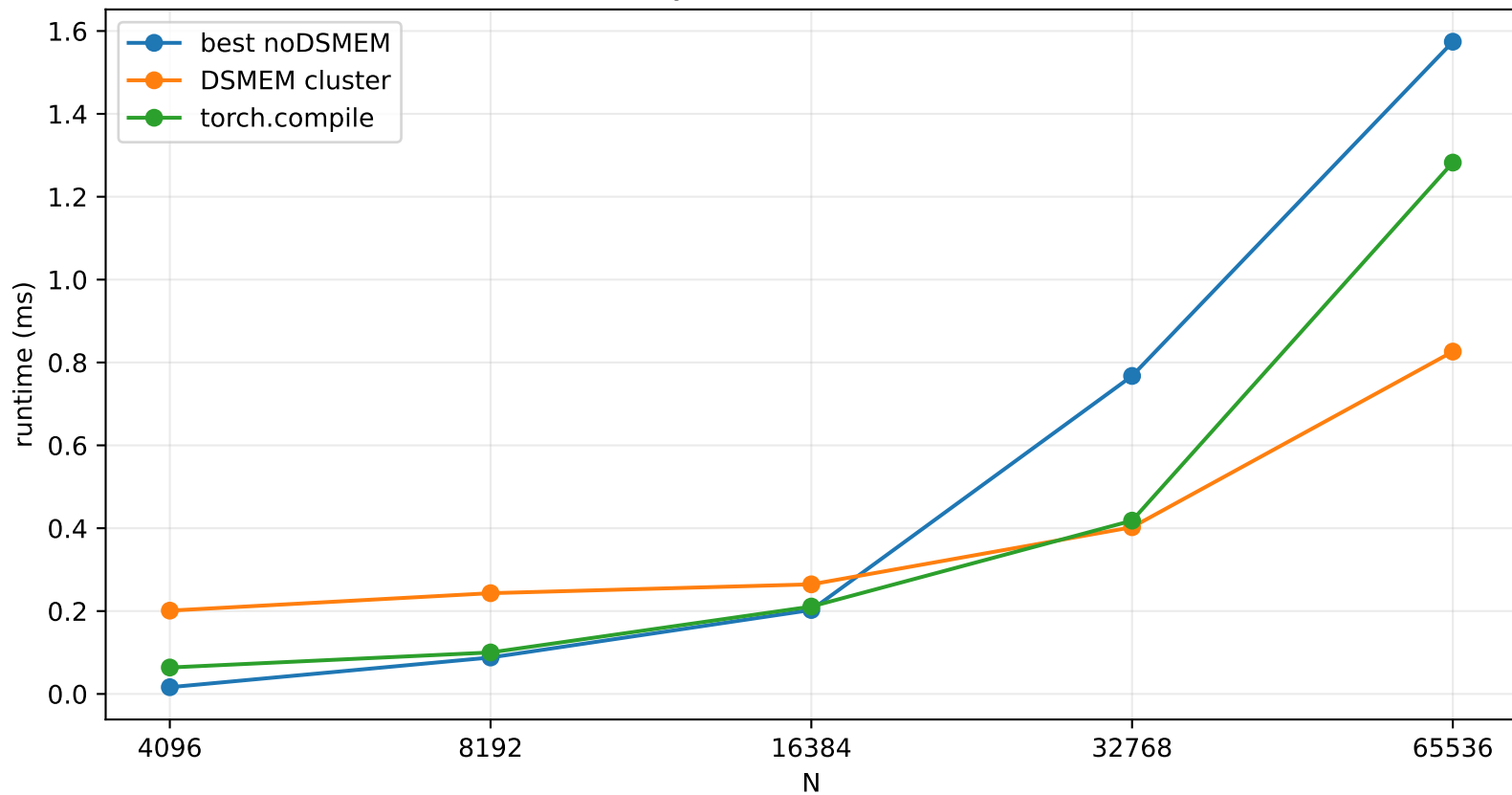
Row-wise Dynamic Quantization Runtime
