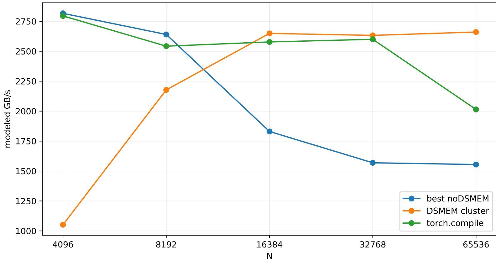
Soft-Target CE Backward Modeled Throughput
