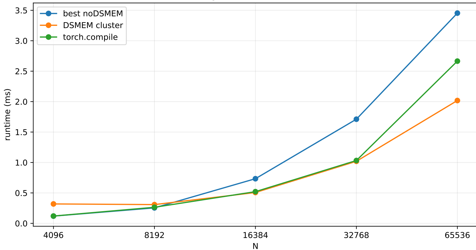
Soft-Target CE Backward Runtime
