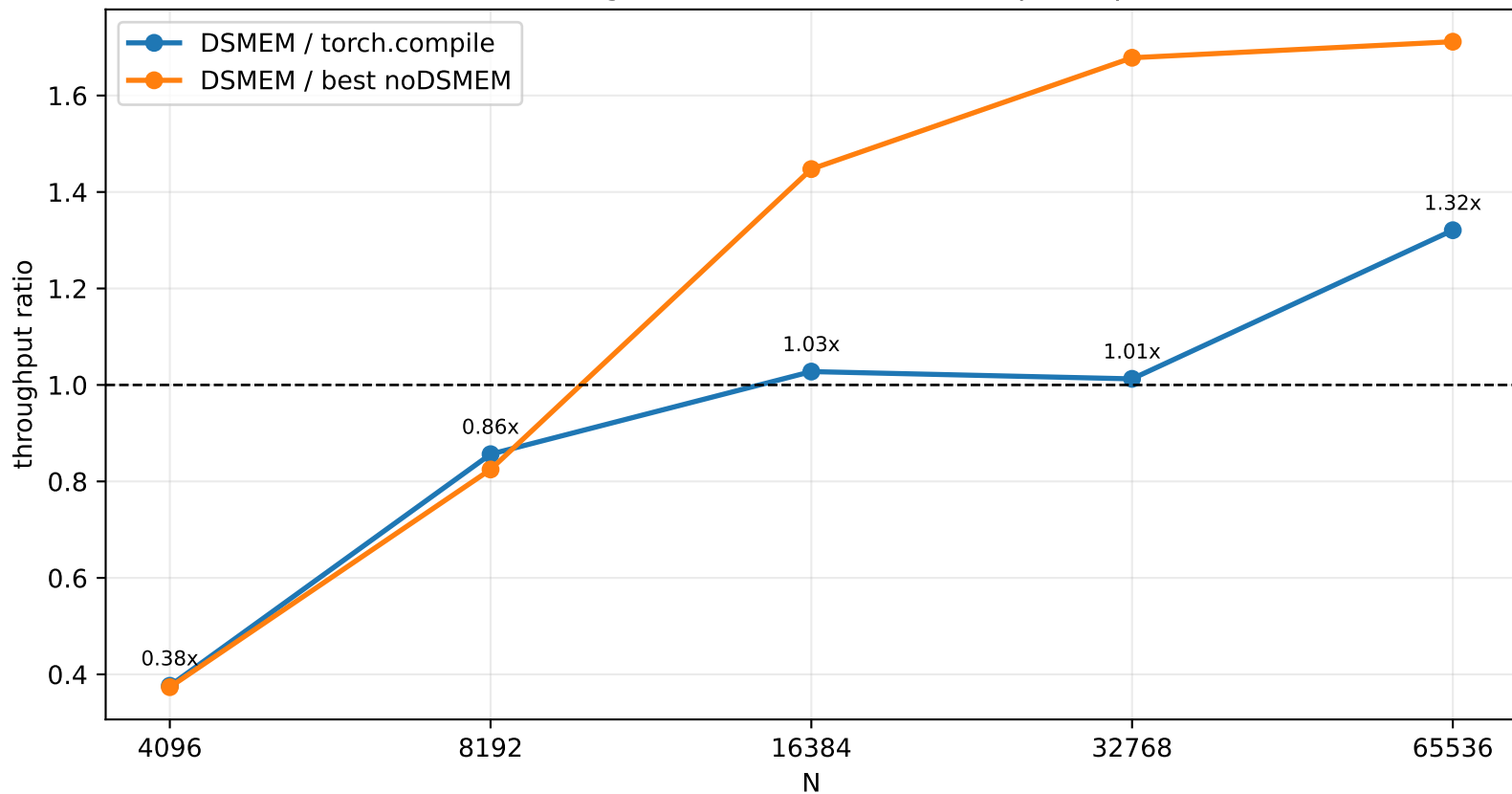
Soft-Target CE Backward DSMEM Speedup
