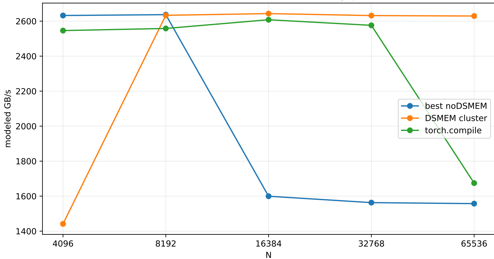
Softmax Backward Modeled Throughput
