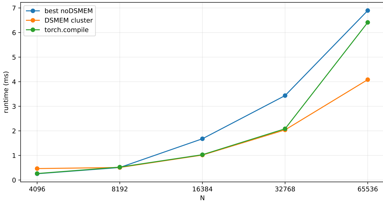
Softmax Backward Runtime
