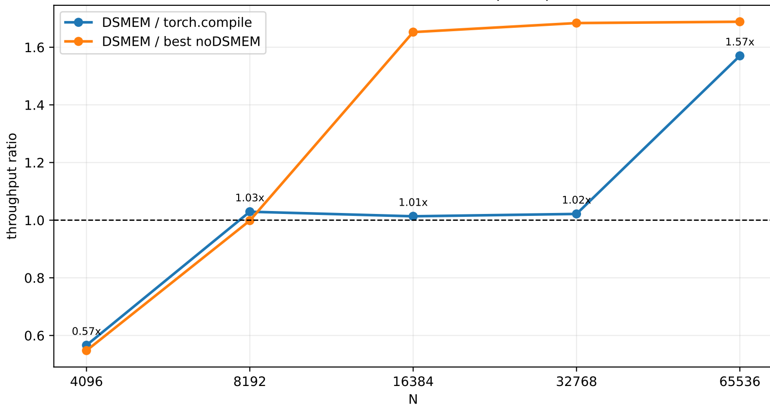
Softmax Backward DSMEM Speedup
