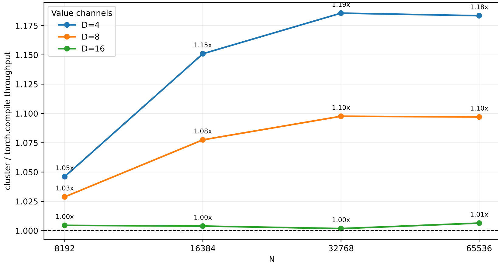
DSMEM Cluster Speedup vs torch.compile
