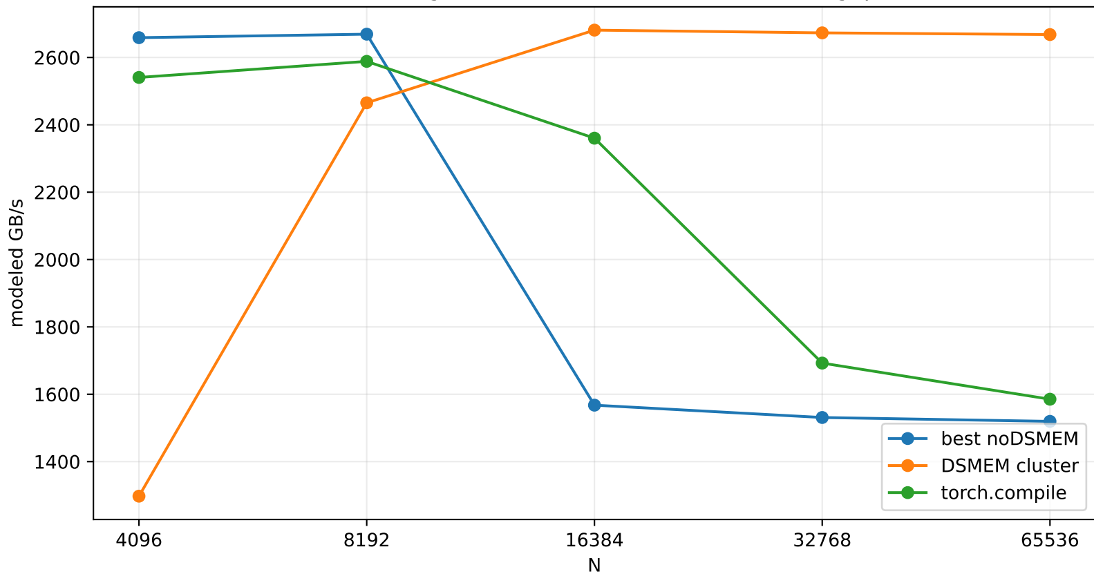
Softmax Weighted Sum Backward Modeled Throughput
