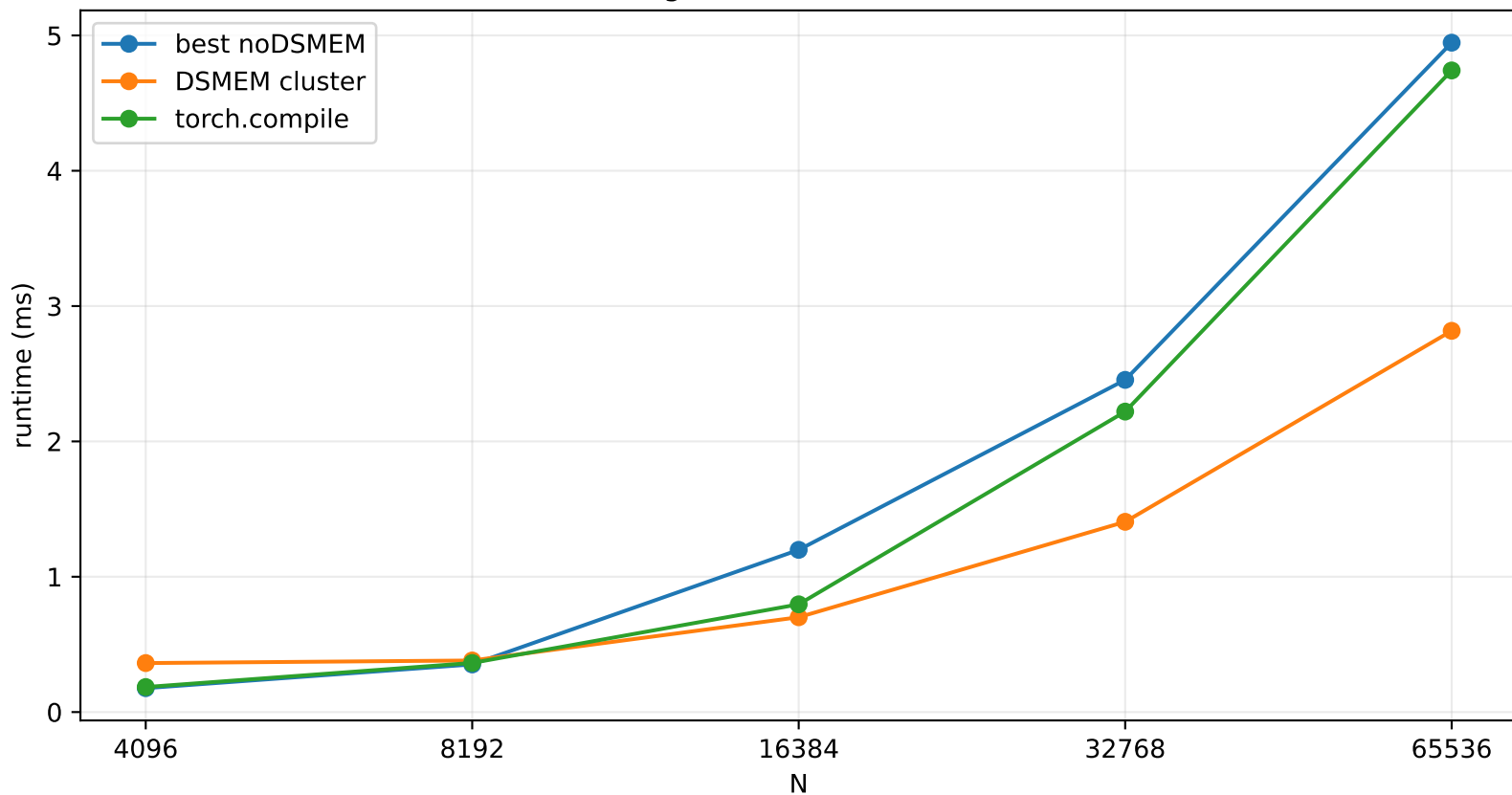
Softmax Weighted Sum Backward Runtime
