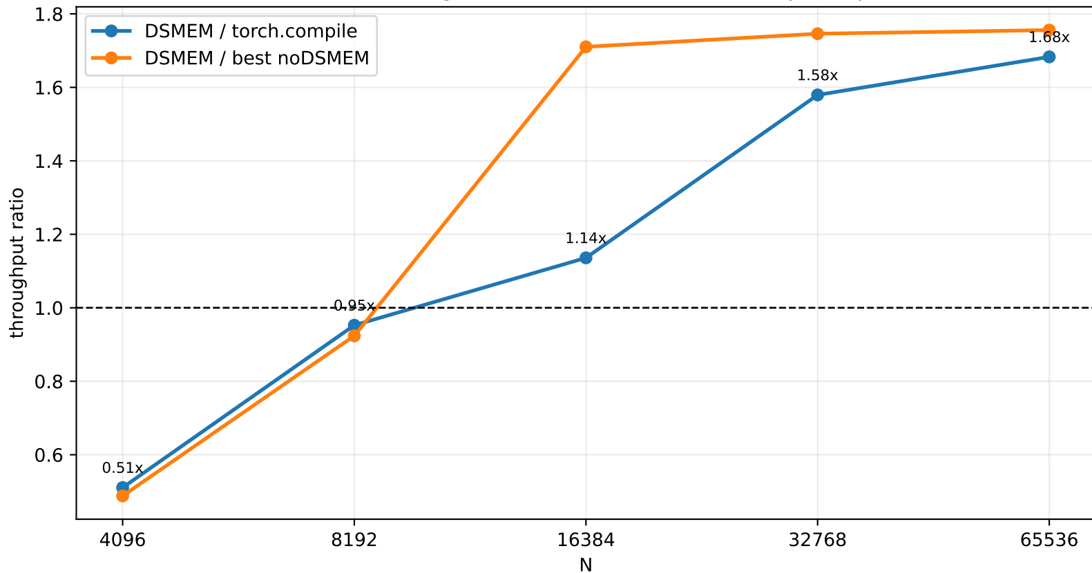
Softmax Weighted Sum Backward DSMEM Speedup
