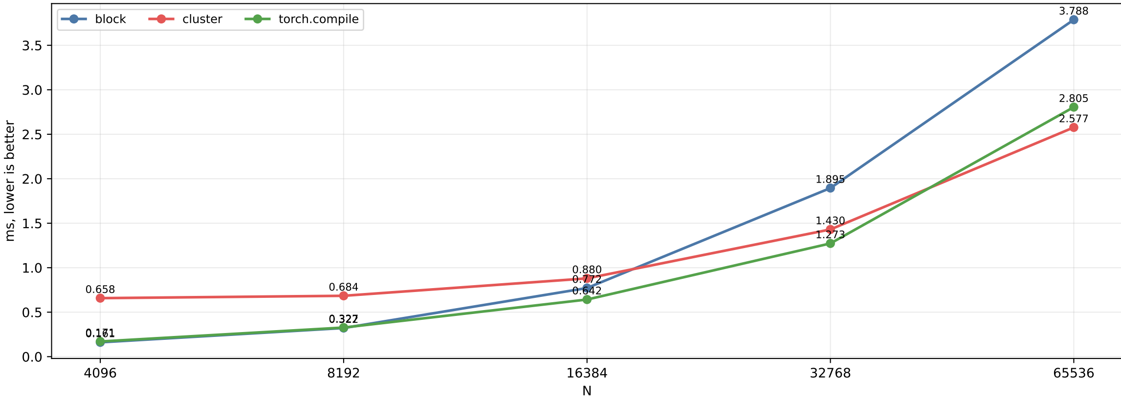
softmax weighted sum: ms, lower is better
