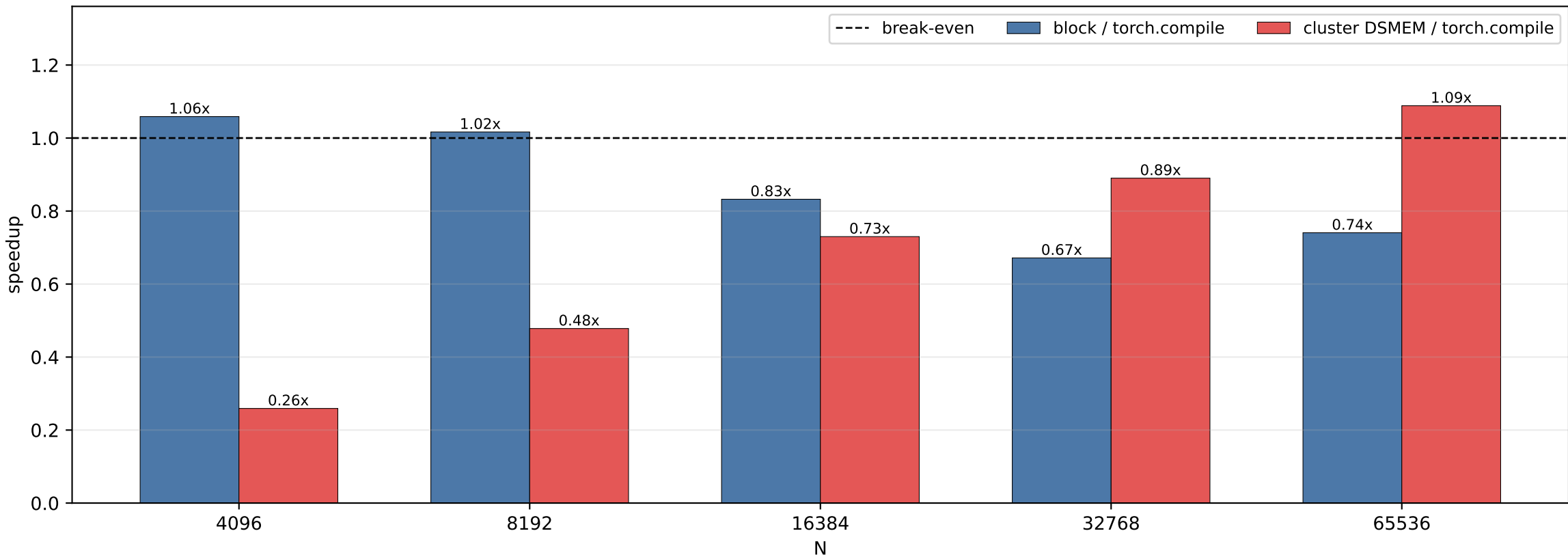
softmax weighted sum: speedup relative to torch.compile
