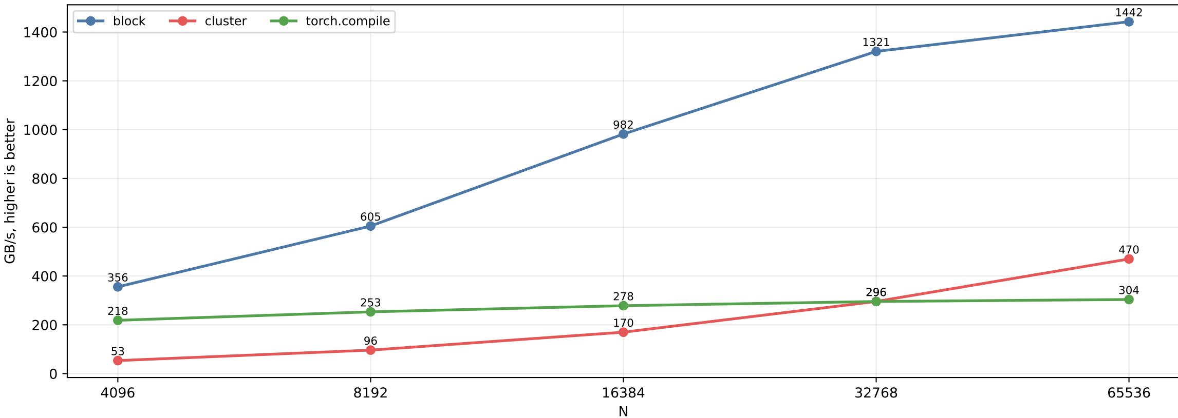
Row-wise top-4: GB/s, higher is better
