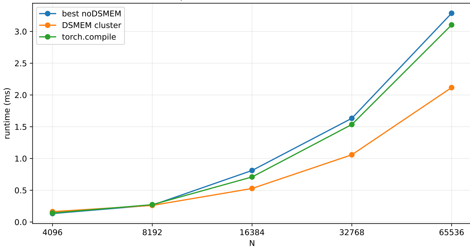
Triplet Distance Backward Runtime
