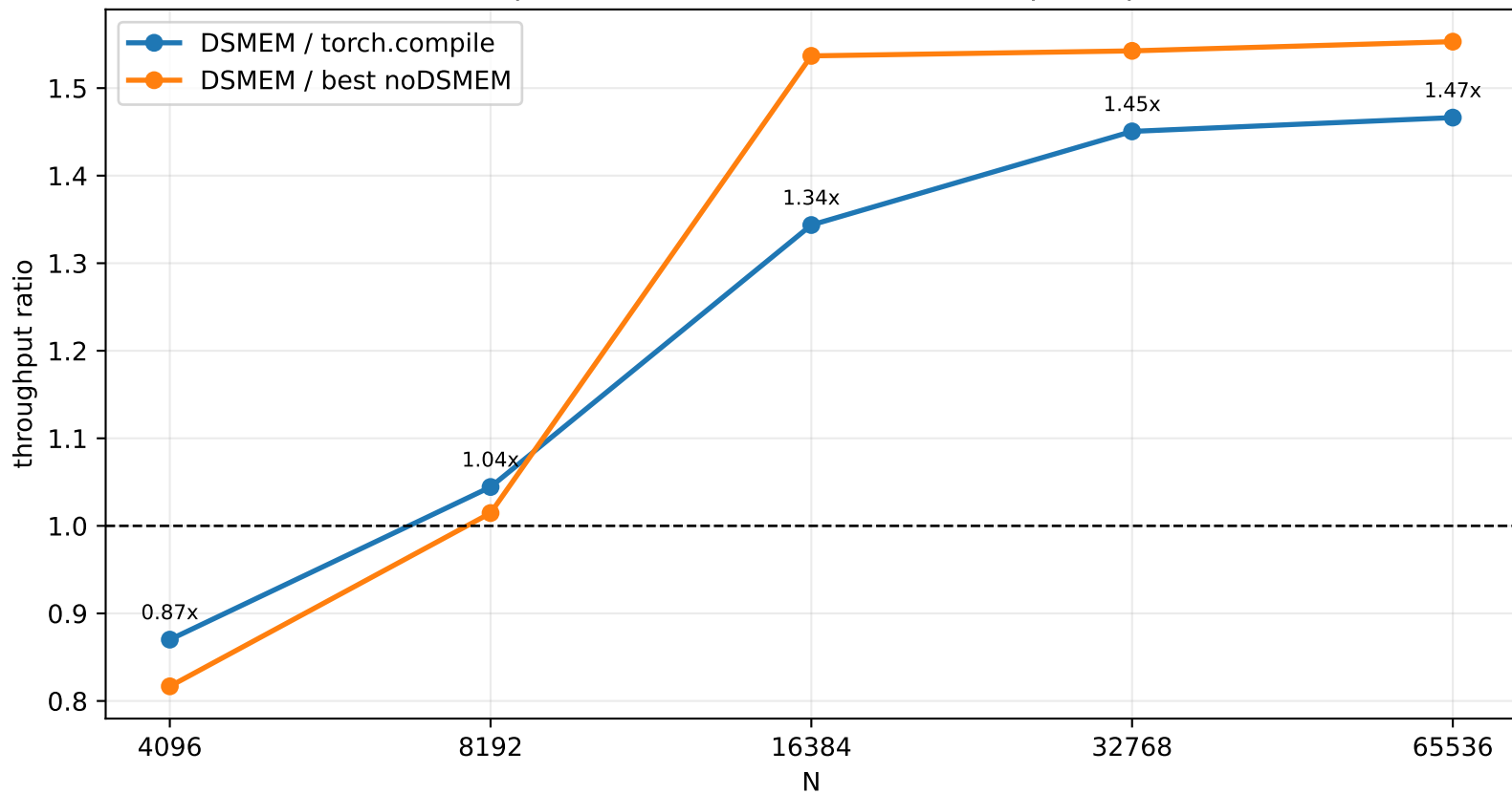
Triplet Distance Backward DSMEM Speedup
