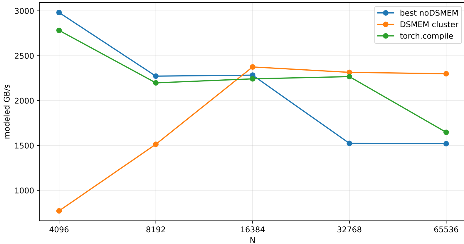
Row-wise Variance Clipping Modeled Throughput
