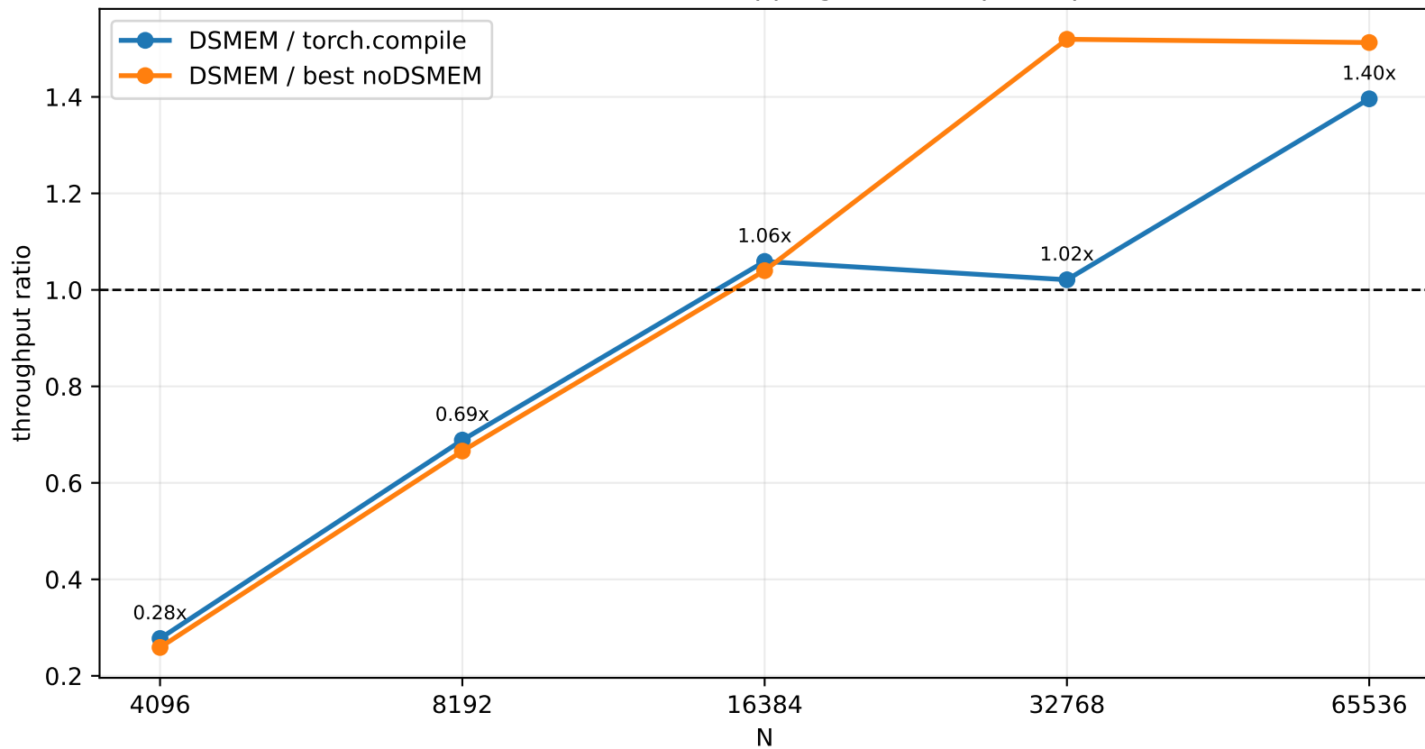
Row-wise Variance Clipping DSMEM Speedup
