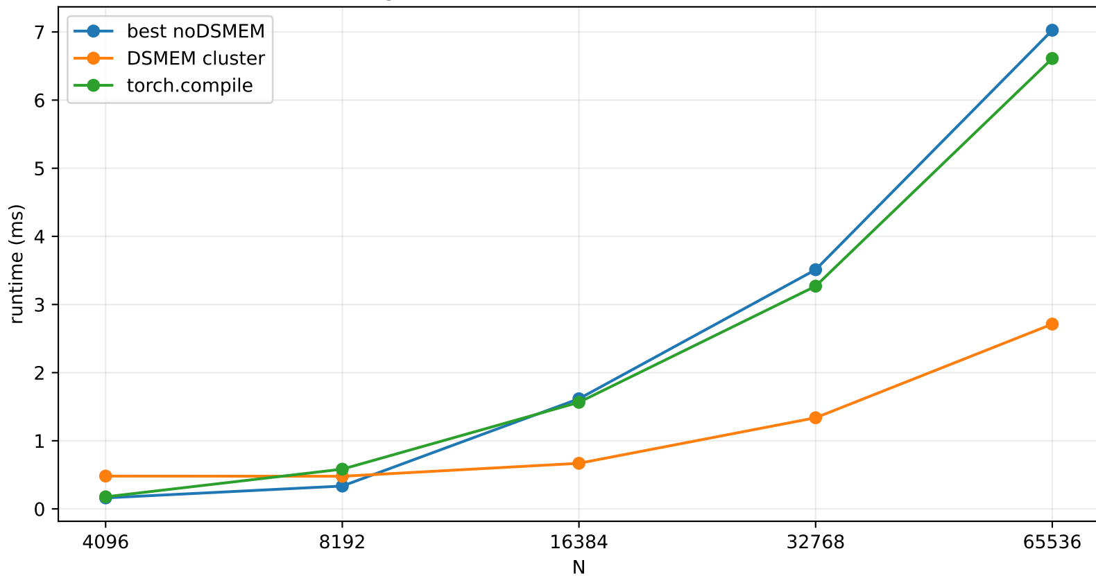
Row-wise Weighted Variance Normalization Backward Runtime
