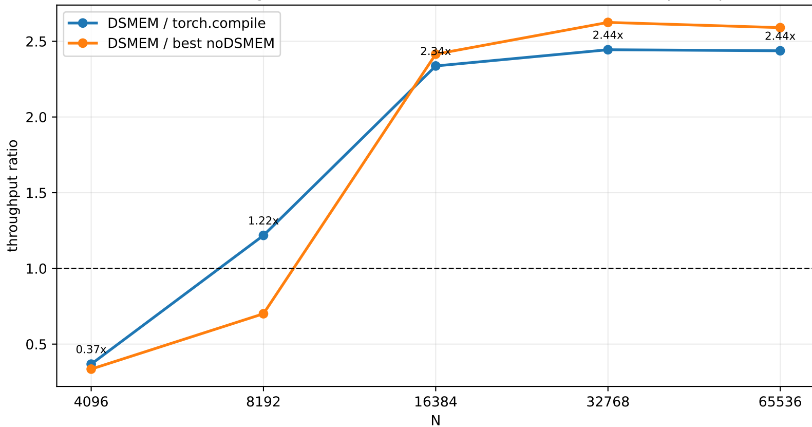
Row-wise Weighted Variance Normalization Backward DSMEM Speedup
