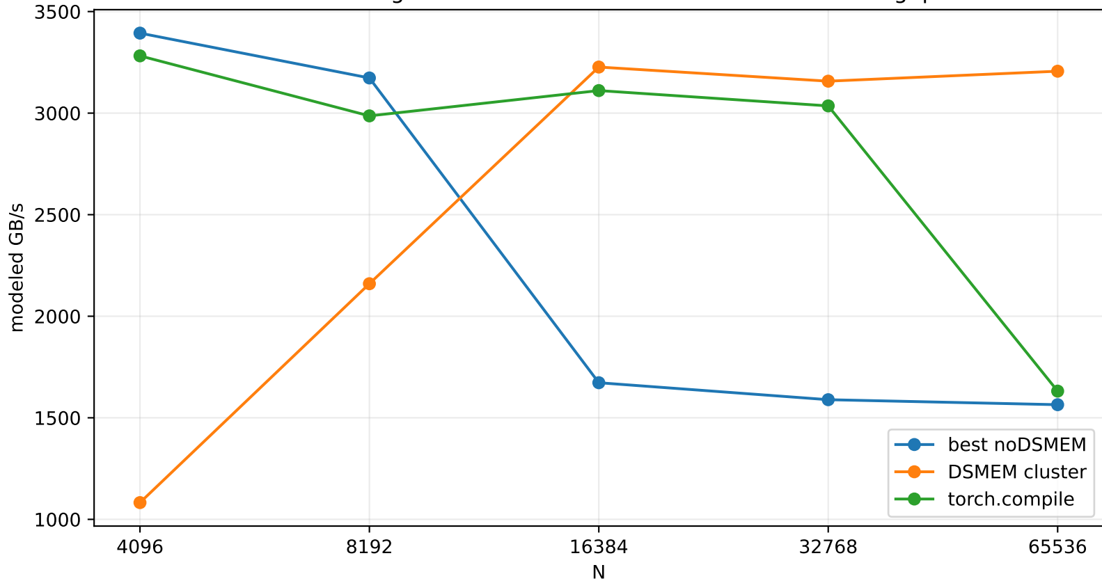
Row-wise Weighted Variance Normalization Modeled Throughput
