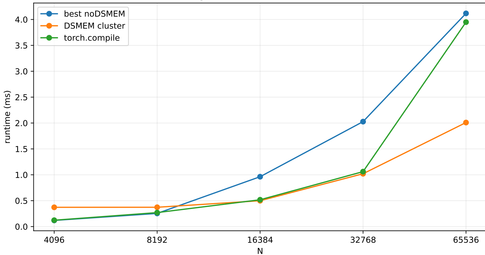
Row-wise Weighted Variance Normalization Runtime
