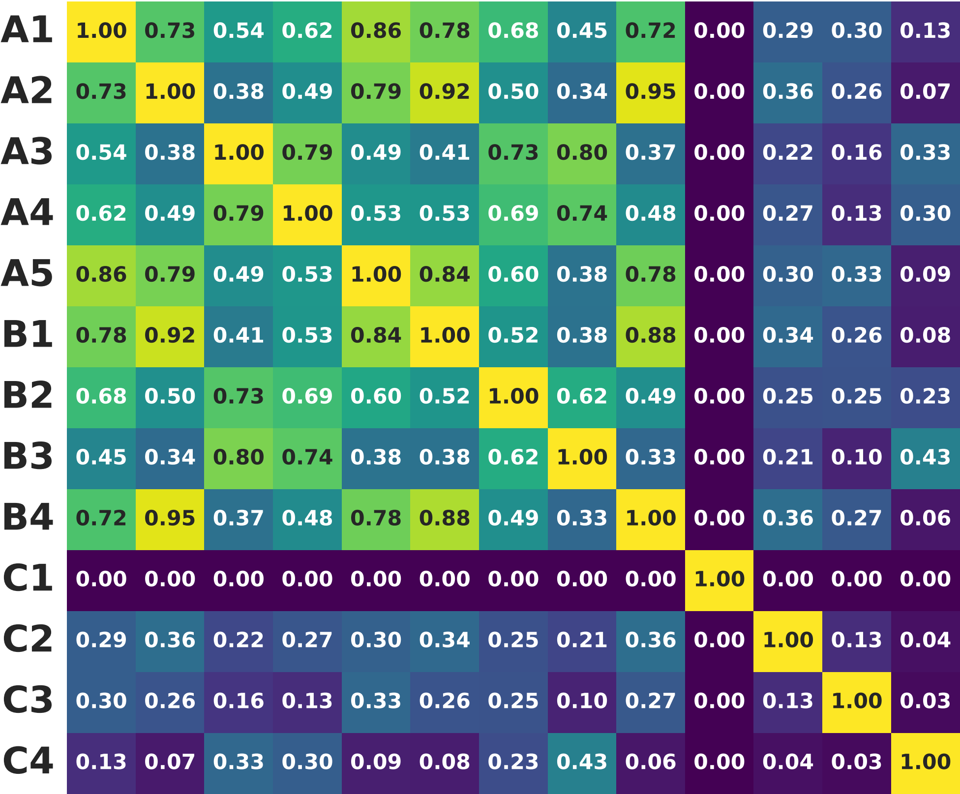
Top-5% (r = 0.05)
