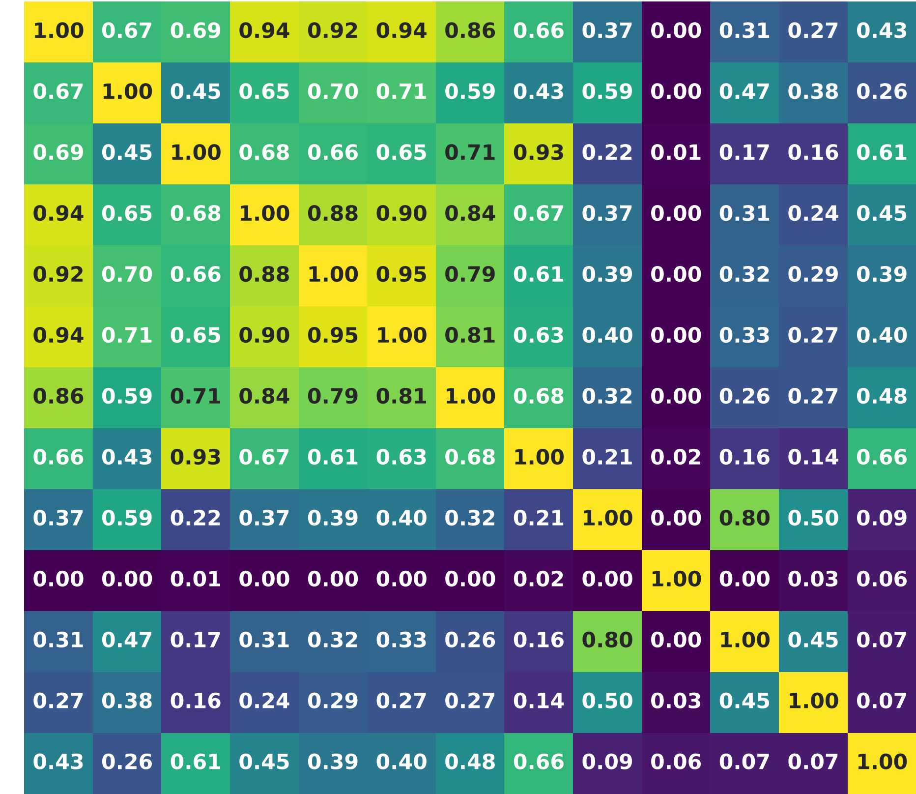
Top-10% (r = 0.10)
