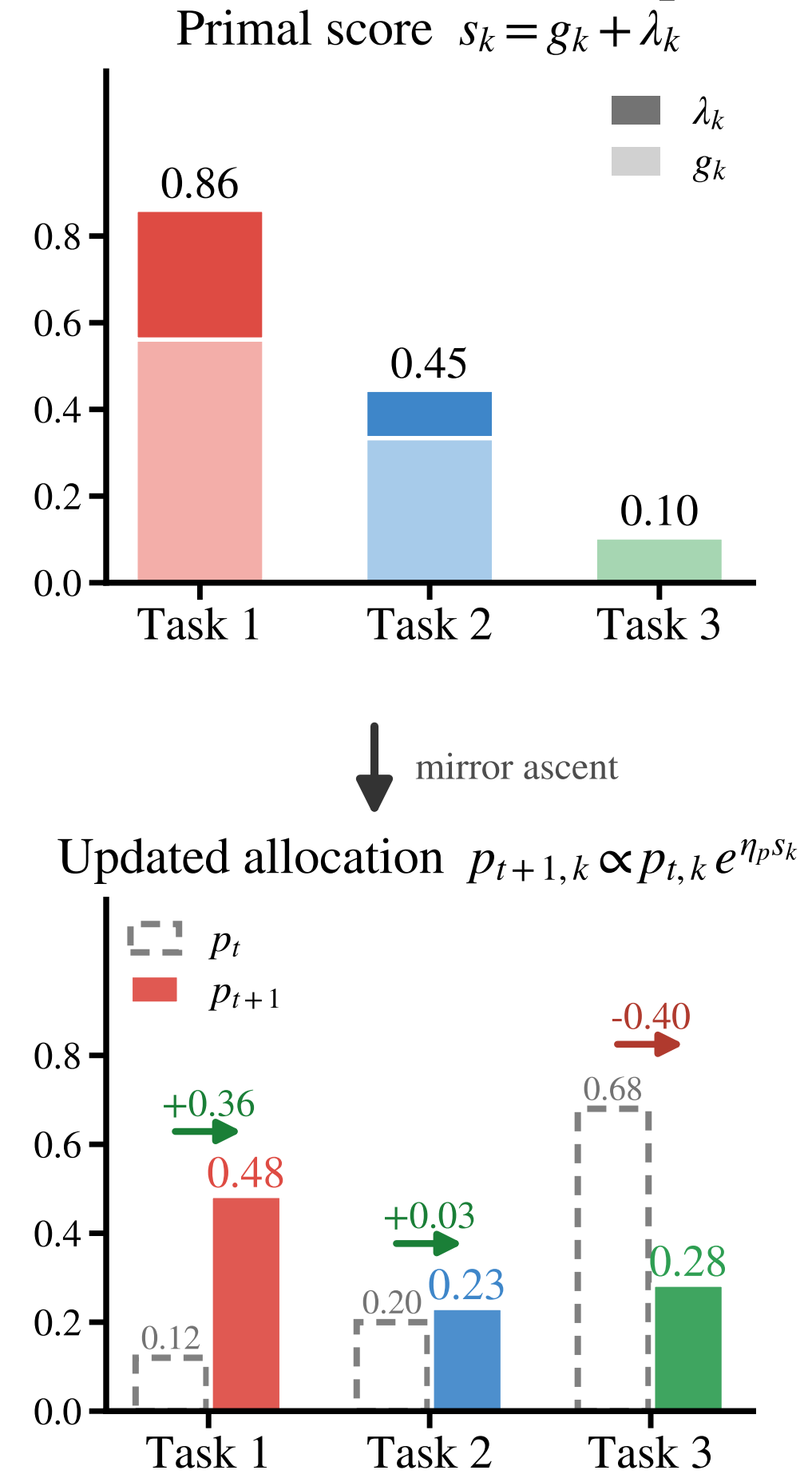
(c) Score and allocation update
