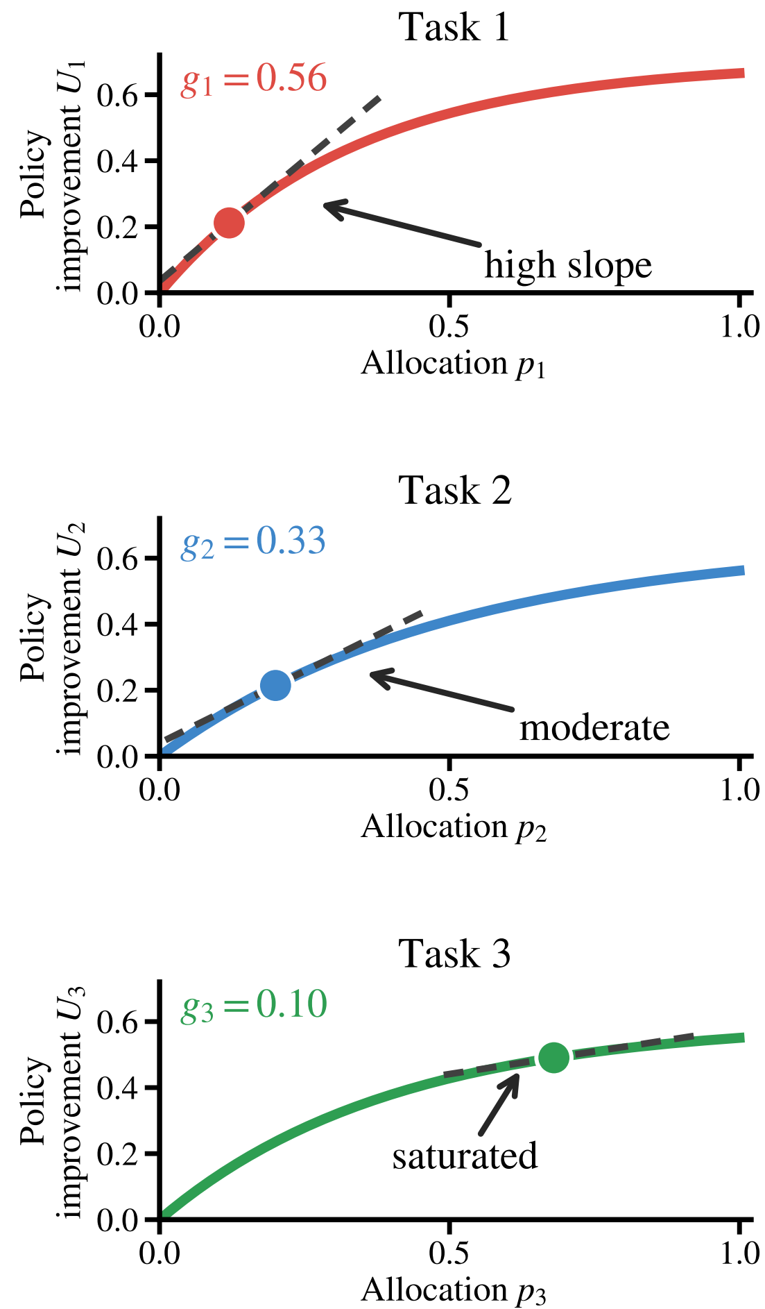
(a) Curvature / marginal improvement
