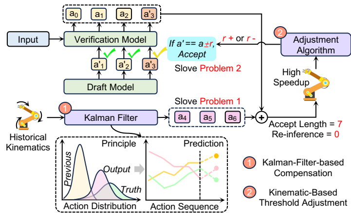
(c) KERV
