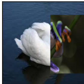
CutMix
