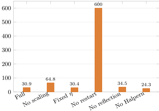
SGM(10) wall time (s)
