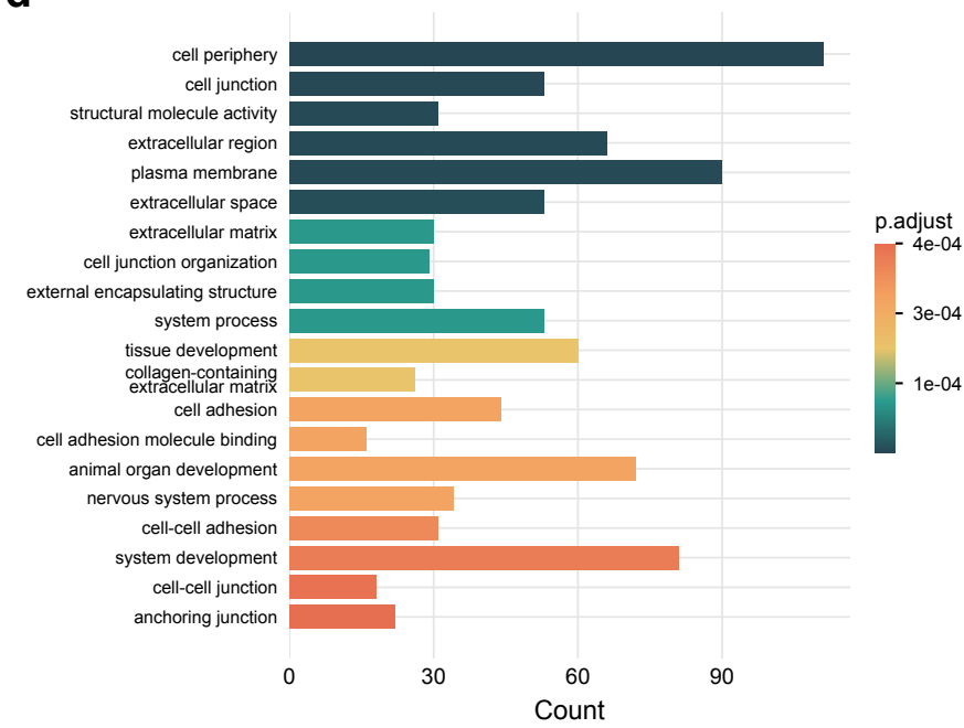
d brain_wave_phase_3_genes.txt - GO (ALL) - Barplot
