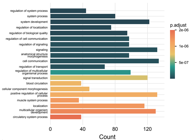
c brain_wave_phase_2_genes.txt - GO (ALL) - Barplot
