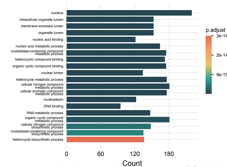
d brain_wave_phase_3_genes.txt - GO (ALL) - Barplot
