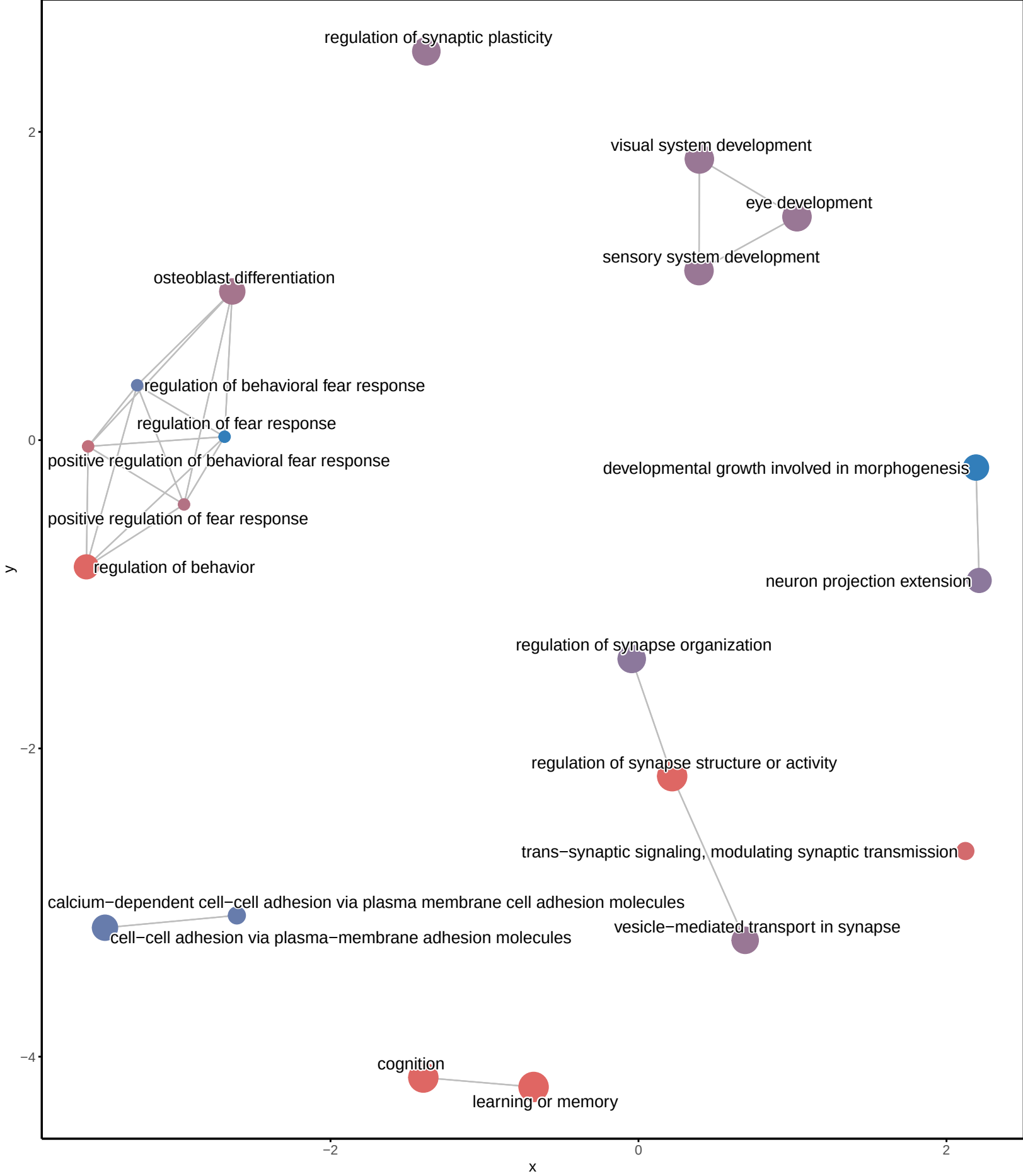
pattern_1_genes.csv – GO (ALL) Enrichment Map
