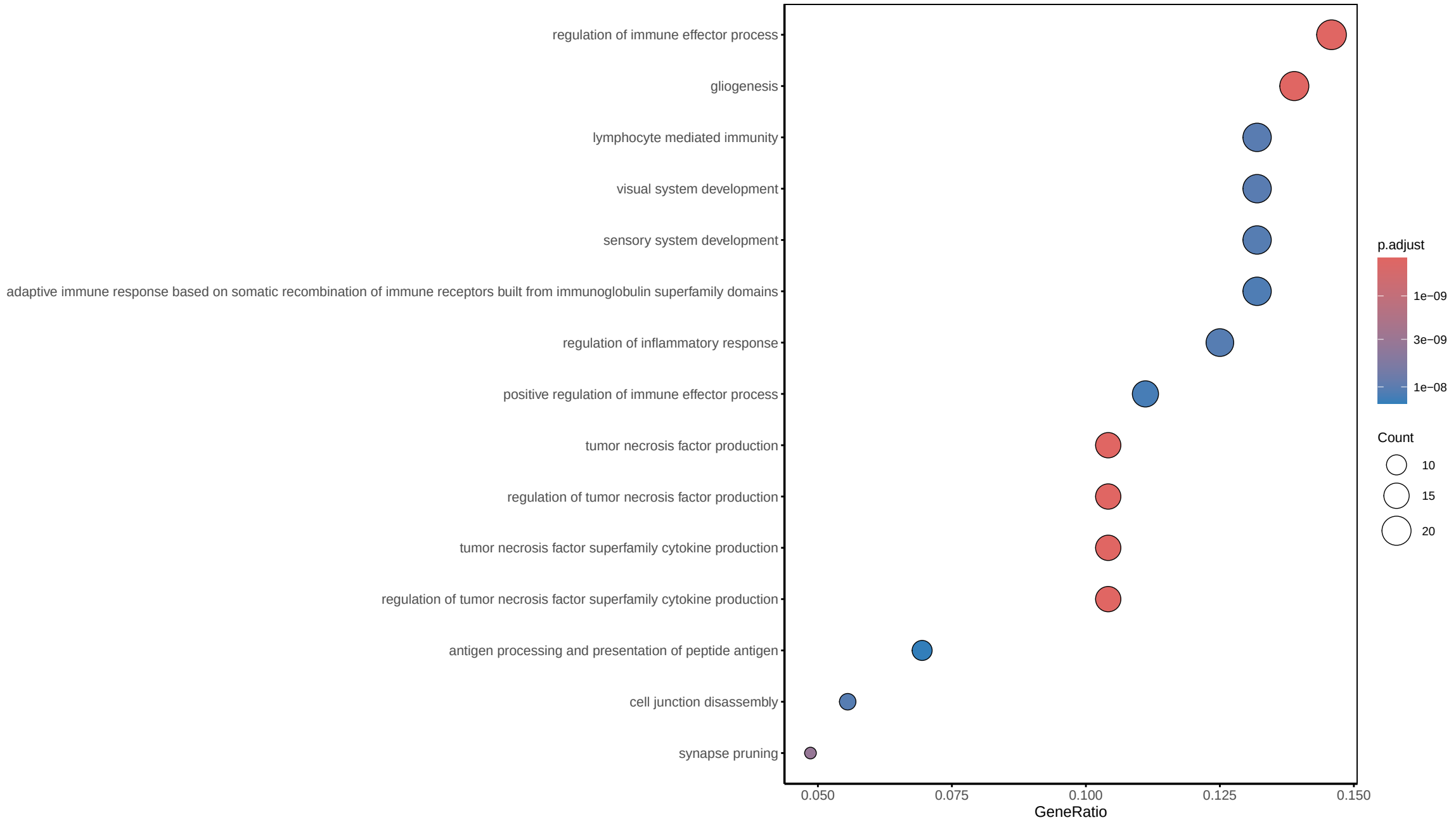
pattern_4_genes.csv – GO (ALL) Dotplot
