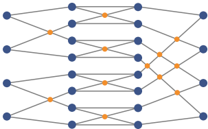
4x4 Dilated Banyan
