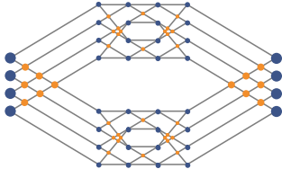
4x4 Double Dilated Benes
