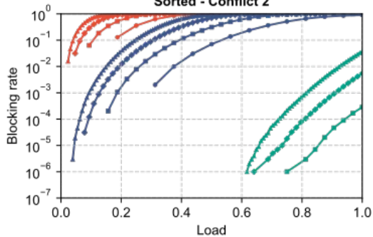
Sorted - Conflict 2
