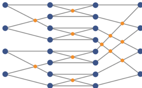
4x4 Dilated Banyan
