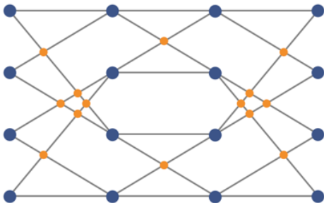
4x4 Dilated Benes
