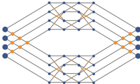
4x4 Double Dilated Benes
