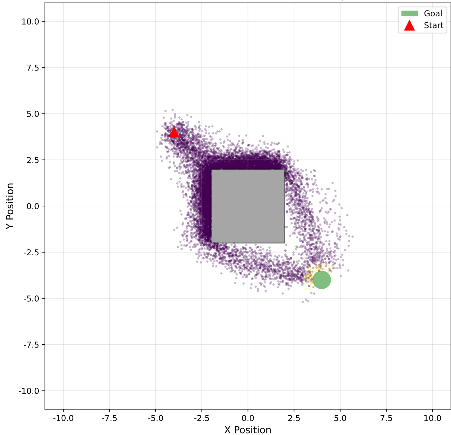
Offline Dataset Distribution in State Space
