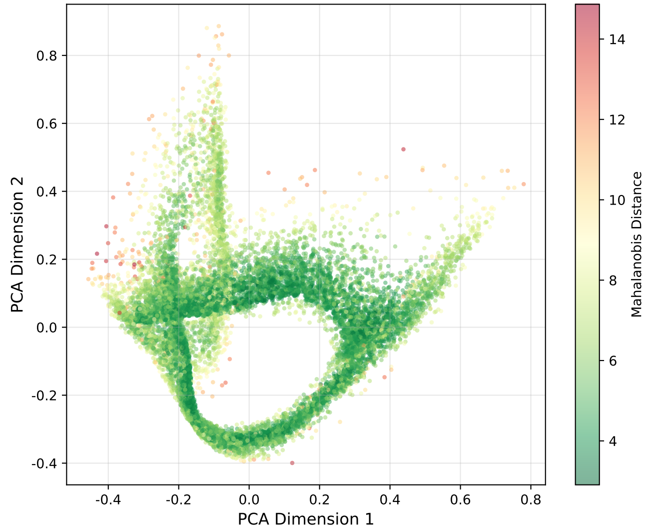
Representation Space (colored by Mahalanobis distance)
