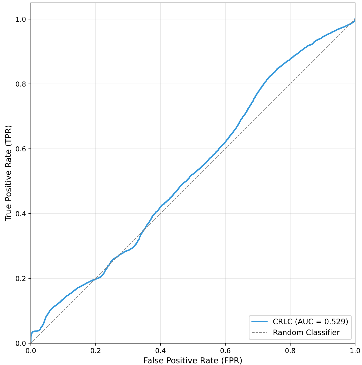
OOD Detection ROC Curve
