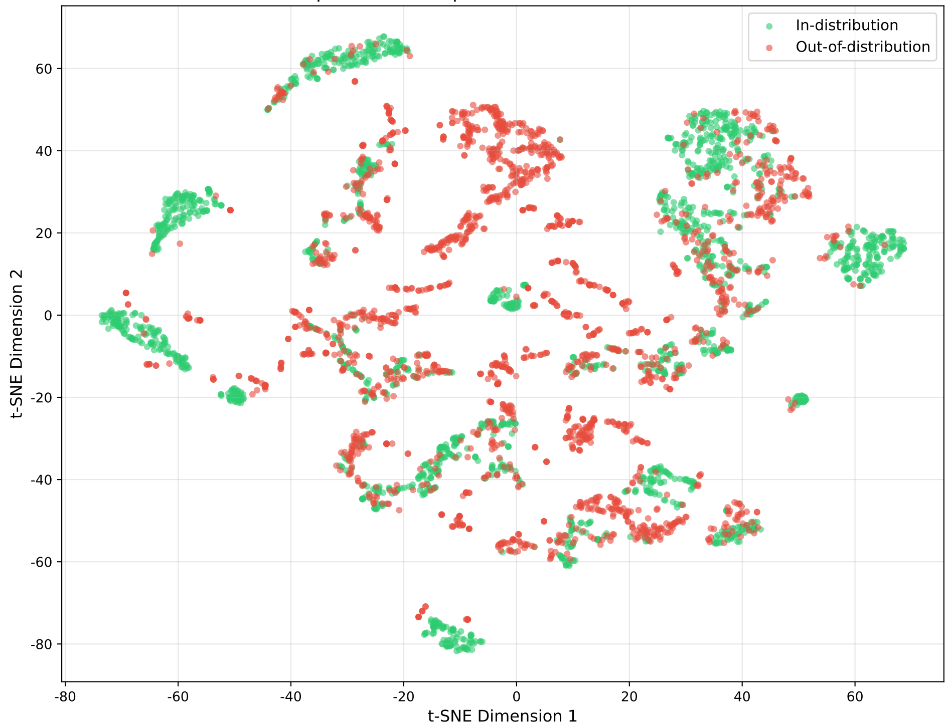
Representation Space Visualization via t-SNE
