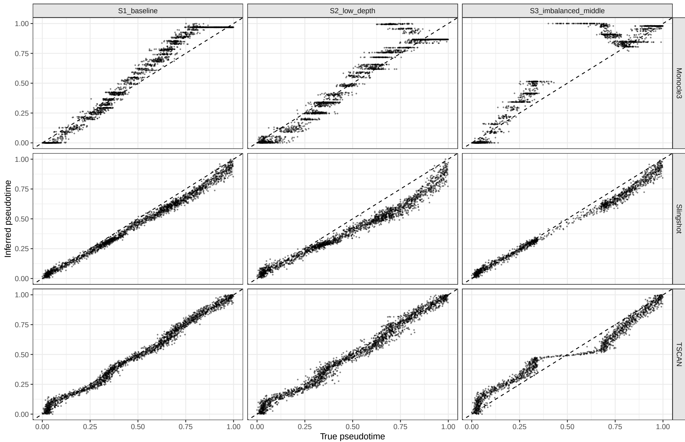
Supplementary Figure 2. True vs inferred pseudotime for all methods and scenarios
