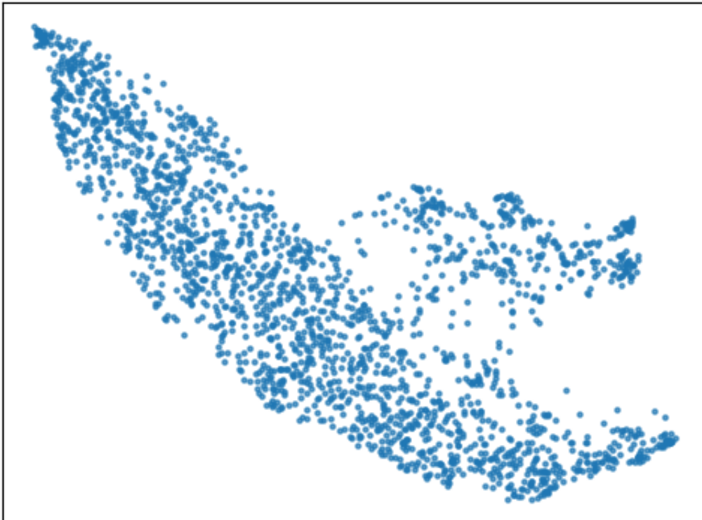
LongSafari/hyenaDNA-large-1m-seqlen-hf
