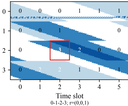
(b) 4-node line OPT=0.585, accepted=1, M_v=3
