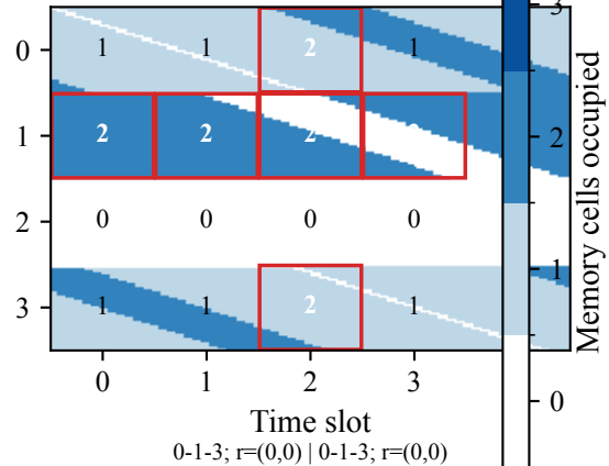
(c) 4-node diamond OPT=1.512, accepted=2, M_v=2
