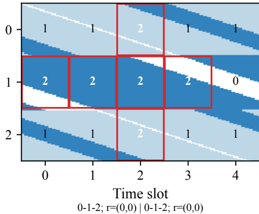
(a) 3-node line OPT=1.457, accepted=2, M_v=2
