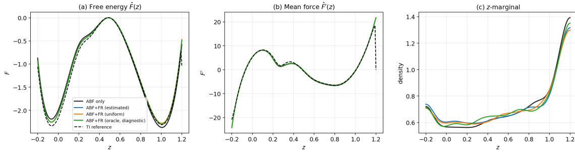
Figure 15: Final profiles (median over seeds) versus the TI reference (dashed): (a) free energy \hat{F}(z) , (b) mean force \hat{F}'(z) , (c) reaction-coordinate marginal. FR recovers the reference free energy more accurately than ABF, chiefly in and around the transition region.
