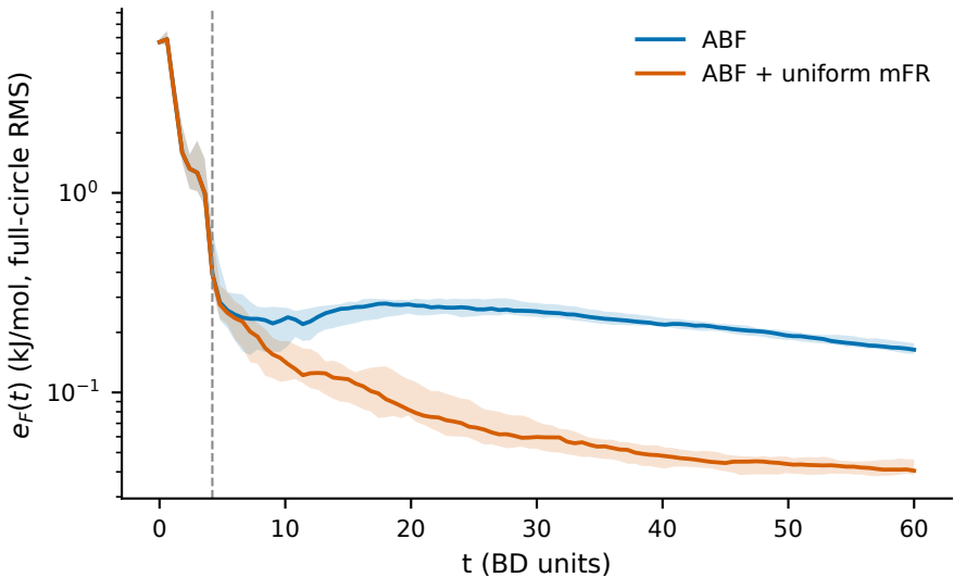
Ethane/LTA 80 K (16 paired seed labels, N=1024)
