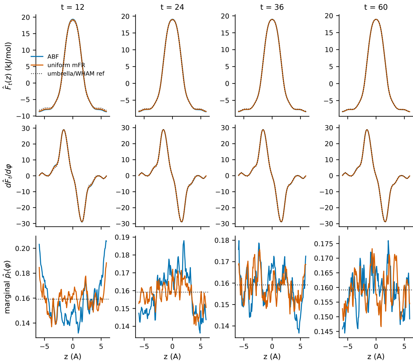
Ethane/LTA: F / mean force / xi-marginal convergence (median over 16 seed labels; window at z=0 , cages at \pm a/2 )
