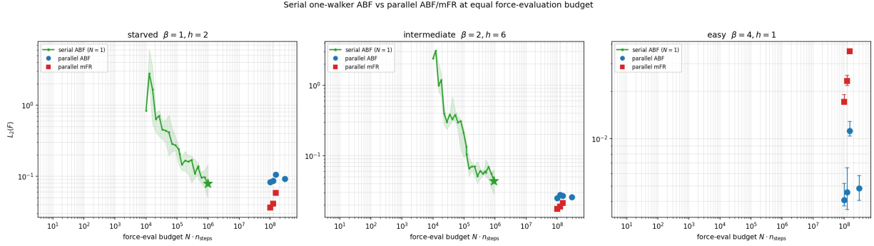
Figure 27: Serial one-walker ABF (green curve, median and IQR over seeds) versus parallel ABF (three N/n_{\text{steps}} shapes) and the deployable mFR at equal force-evaluation budget B = N \cdot n_{\text{steps}} , for the starved, intermediate and easy cells. The dotted line marks the base equal budget 1024 \times 120\text{k} . Serial ABF is drawn along its accumulated budget so its plateau (or catch-up) is visible; the parallel methods are points at their budgets.
