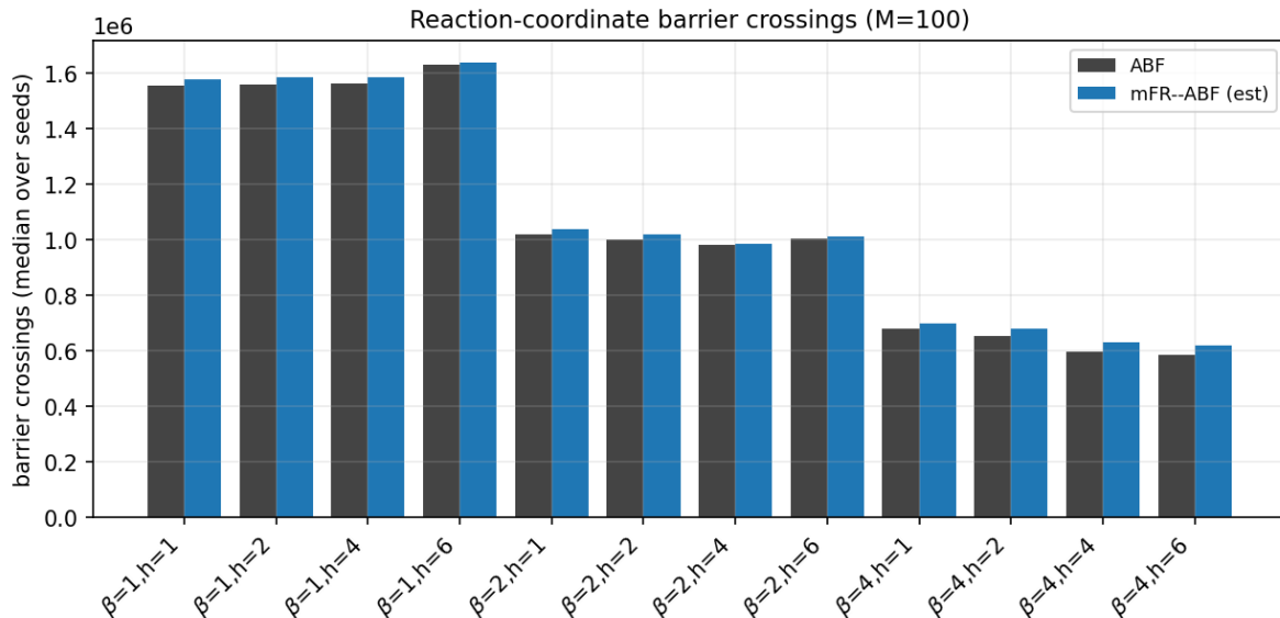
Figure 19: Barrier-crossing counts for ABF and mFR-ABF (estimated target) in the same production cells. mFR slightly increases crossing counts in most cells, but the accuracy gain does not follow crossing count alone: unnecessary resampling can raise crossings while worsening L^2(F) when ABF is already accurate.
