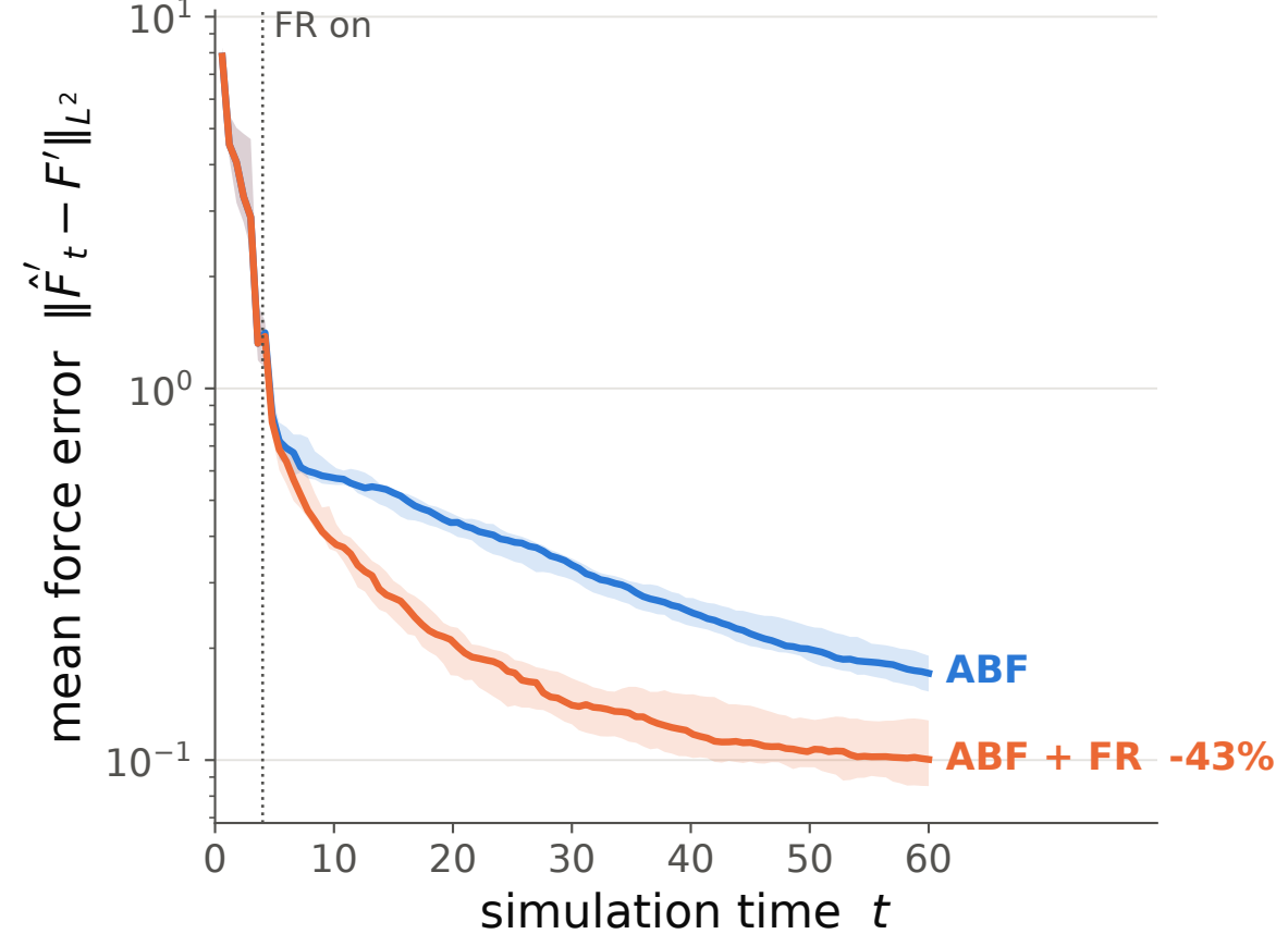
Mean force
