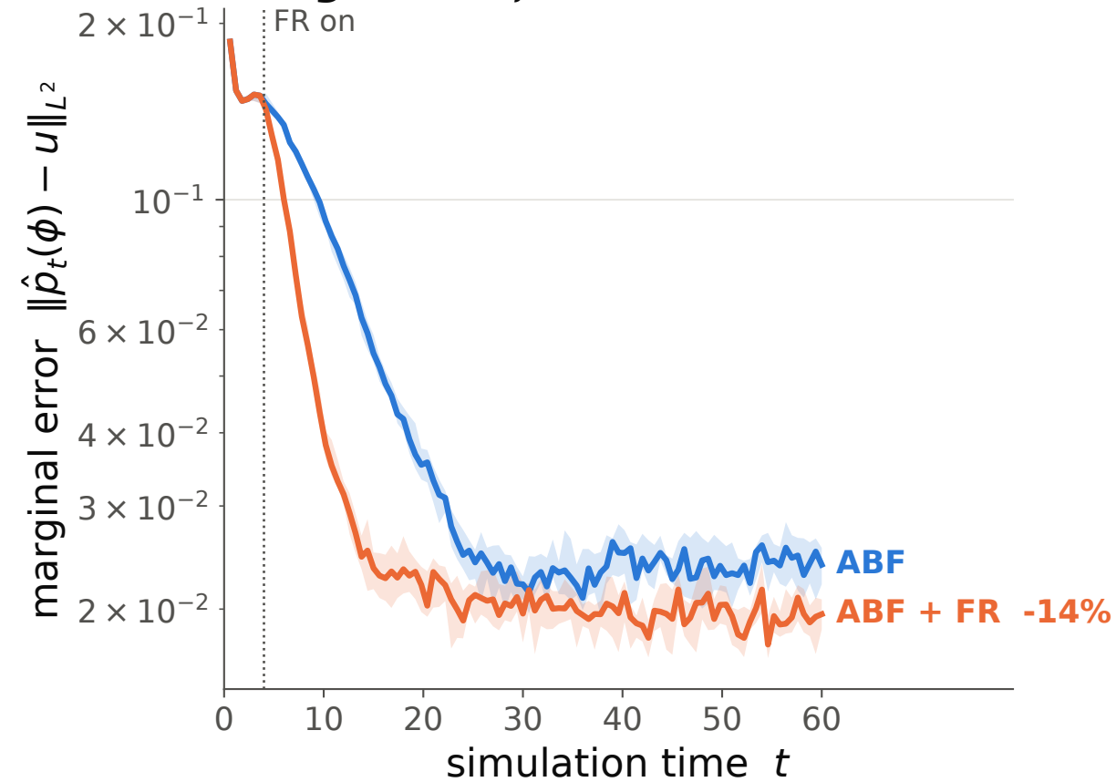
Marginal of \xi
