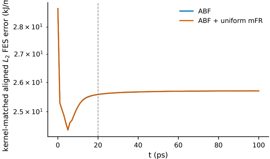
Alanine (vacuum), 16 paired seeds, N=2048
