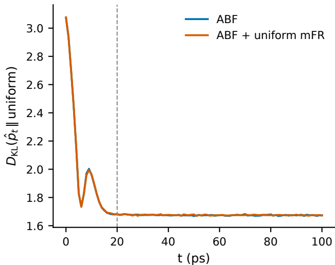
marginal establishment on the torus
