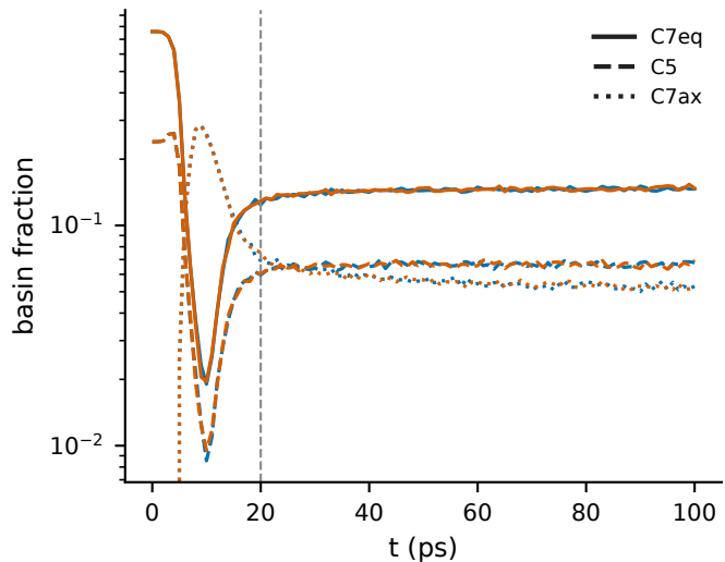
basin occupancy (blue=ABF, red=uniform mFR)
