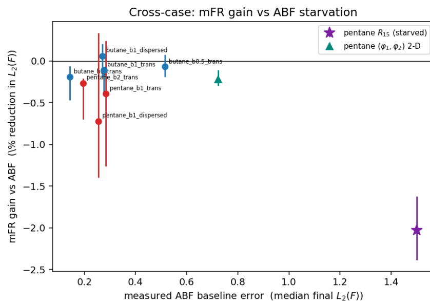
Figure 50: Cross-case starvation map: matched-seed mFR gain versus measured ABF baseline error, with the butane and pentane \varphi_1 points overlaid on the WCA regime cells (grey). The collective-variable extension adds the two decisive points: the pentane R_{15} cell (purple star) sits at the largest measured ABF error anywhere in the study yet returns a negative mFR gain, and the 2-D torsion cell (teal triangle) is likewise flat. The WCA-derived reading — that measured ABF error predicts mFR gain — therefore does not extrapolate to molecular coordinates: high ABF error is necessary but not sufficient, because R_{15} starvation is dynamical (rare barrier crossing) rather than a marginal support deficit that reallocation can repair.
