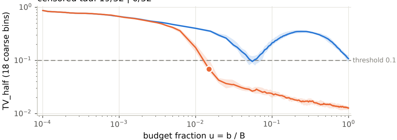
(a) TV_half: visitation over the trailing half C_{\text{all}}(t) - C_{\text{all}}(\approx t/2) censored tau: 19/32 | 0/32
