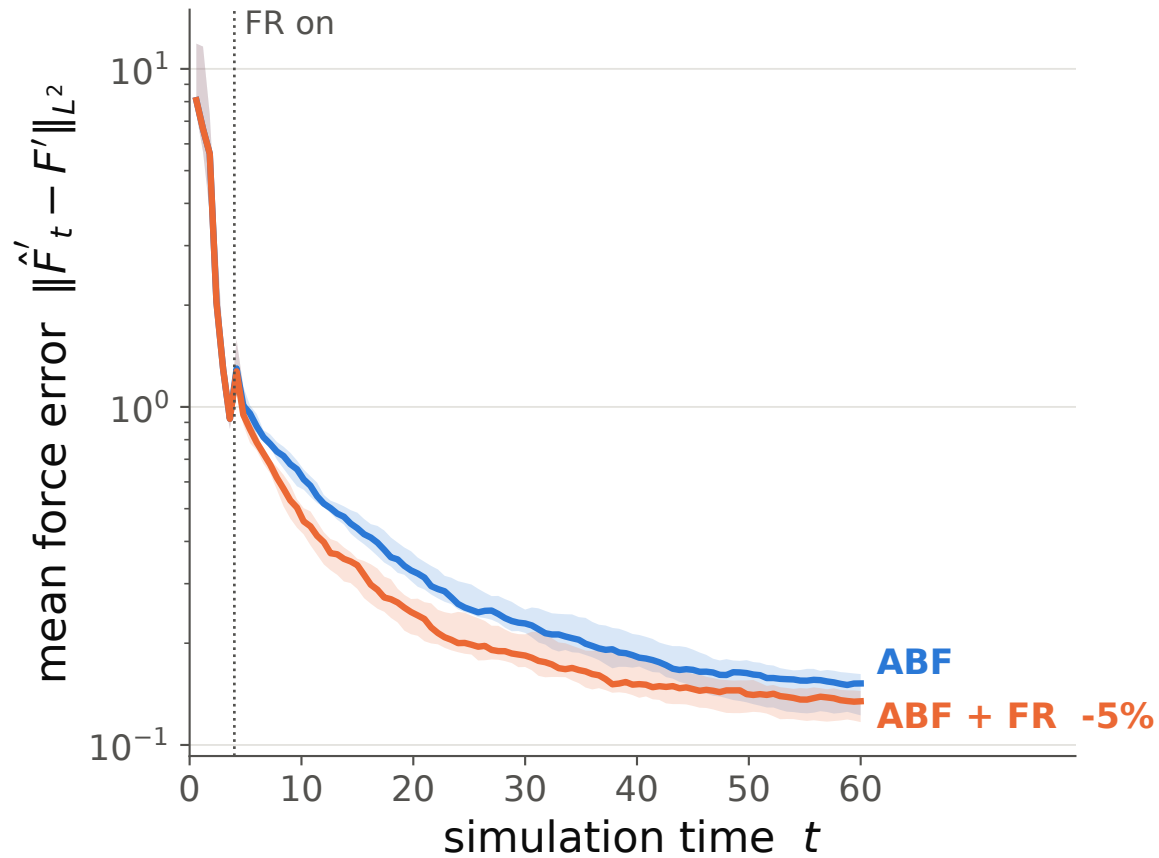
Mean force
