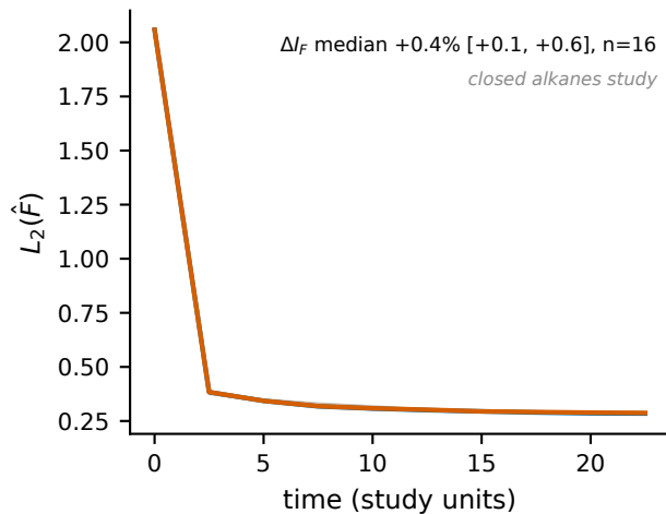
Pentane \phi_1 (trans, \beta=1 )
