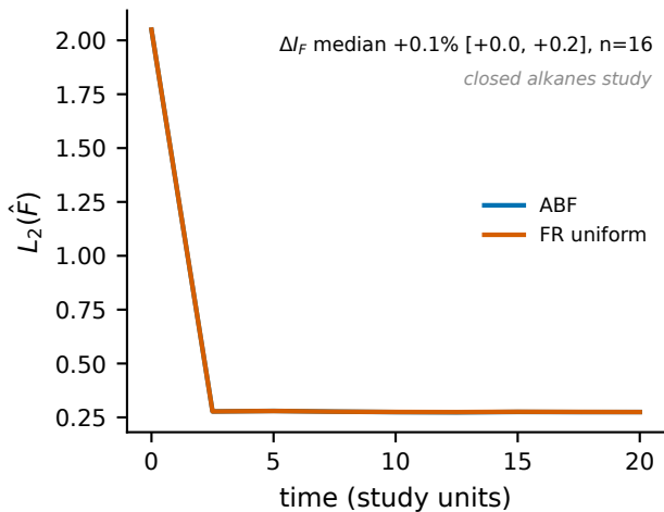
Butane \phi_1 (trans, \beta=1 )
