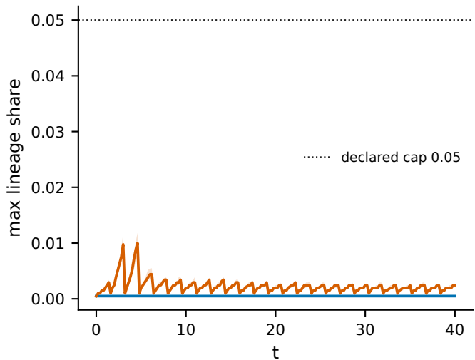
Gateway genealogy (init: left; 4000-step ancestry window)
