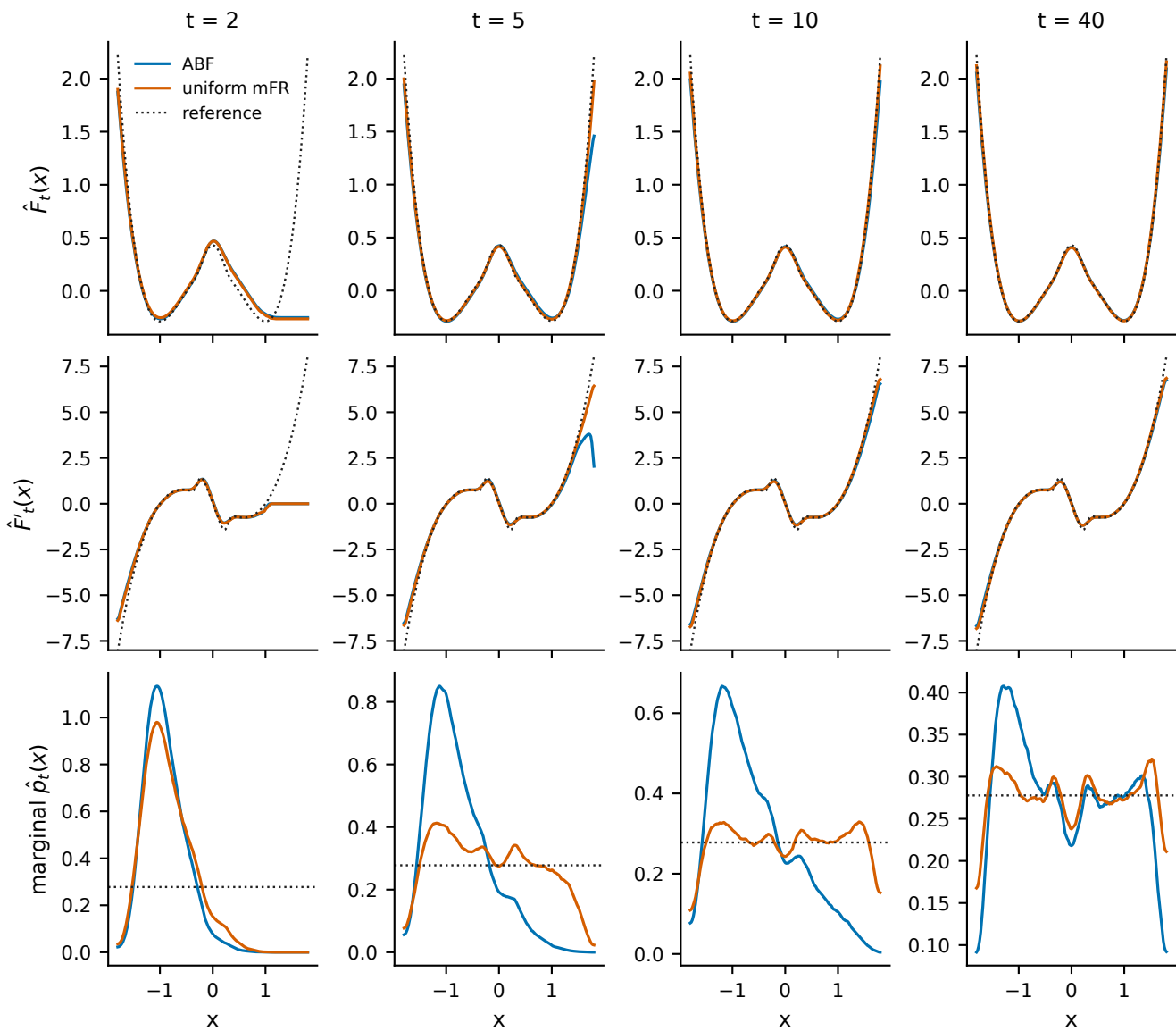
Gateway: F / mean force / xi-marginal convergence (median over 32 seeds, init: left; dotted = reference / uniform)
